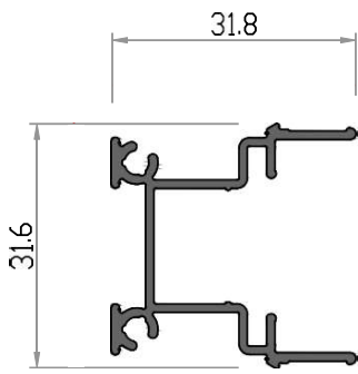
Inner Cartridge
