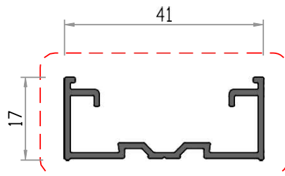
Bottom Rail
