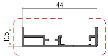
Catch Frame
