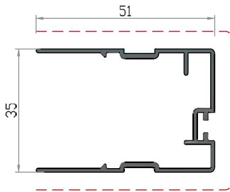
Sliding Bar
